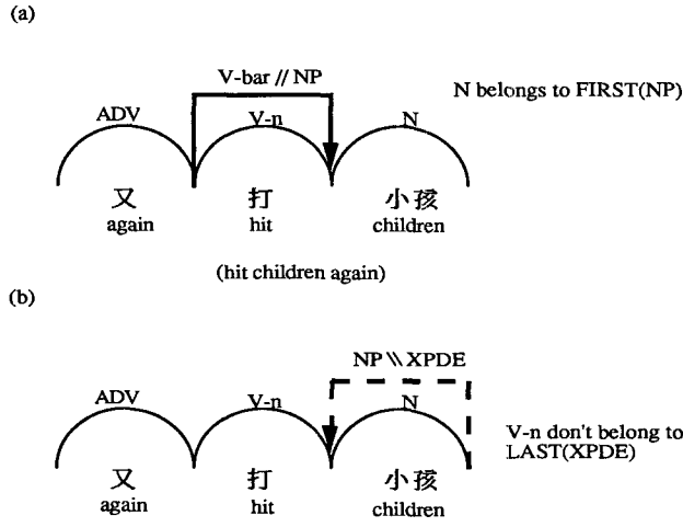
Figure 10 An example to illustrate the use of FIRST and LAST parsing tables to avoid building many unnecessary active edges on the direction-selective chart.
