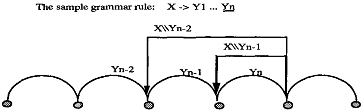
Figure 5 The searching actions in the direction-selective chart.
